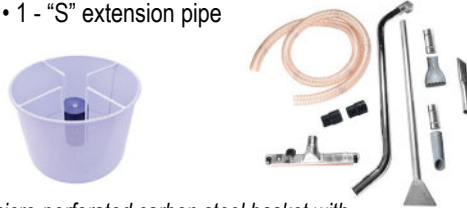
micro-perforated carbon steel basket with added 150 micron PPL filter for very fine chips
