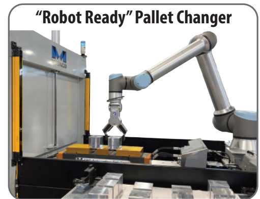
Shown with optional Trunnion System for 4th-axis milling on VMC with 1 rotary indexer
