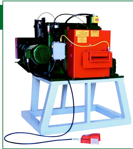
The Model 5403 is shown with an optional stand. Sweed Machinery offers a number of stand/container options.
