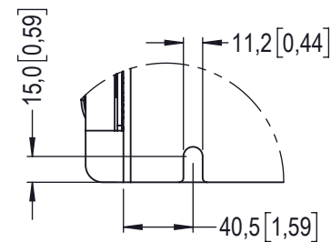
DETALHE/DETAIL B ESCALA/SCALE 1 : 4
