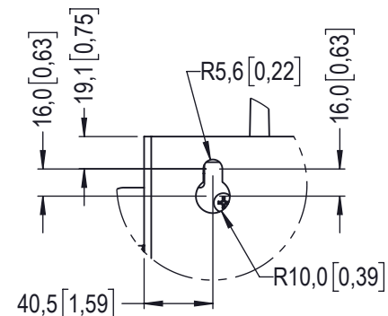
DETALHE/DETAIL A ESCALA/SCALE 1 : 4
