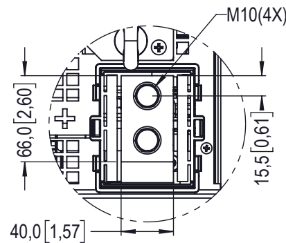
DETALHE/DETAIL C ESCALA/SCALE 1 : 4
