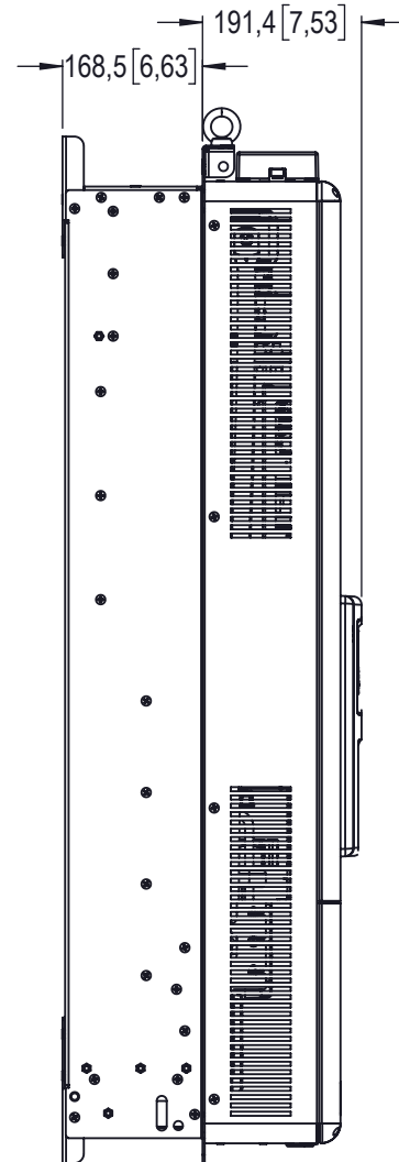
DETALHE/DETAIL A ESCALA/SCALE 1 : 4
