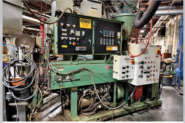
3.5" Davis Standard NRM Extruder w/ High Technology Screen Changer
